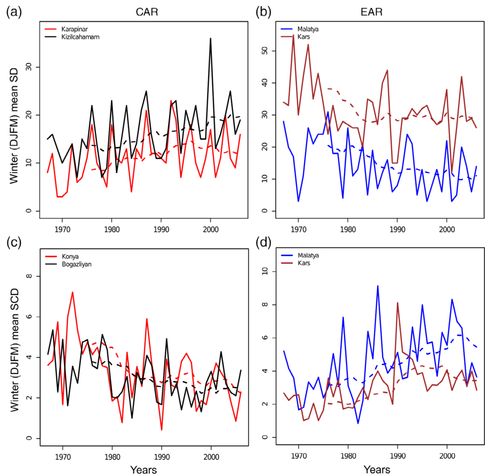
FIGURE 3 Temporal behaviour of winter mean (a), (b) snowy days (SDs) and (c), (d) snow cover depth (SCD). Karapinar, Kizilcahamam, Konya, Bogazliyan (Malatya, Kars) stations in the left (right) panels are used for their high positive (negative) SD trends in the central Anatolia region (CAR) (eastern Anatolia Region [EAR]). The dashed lines indicate the 10 year moving average; DJFM, December–March
