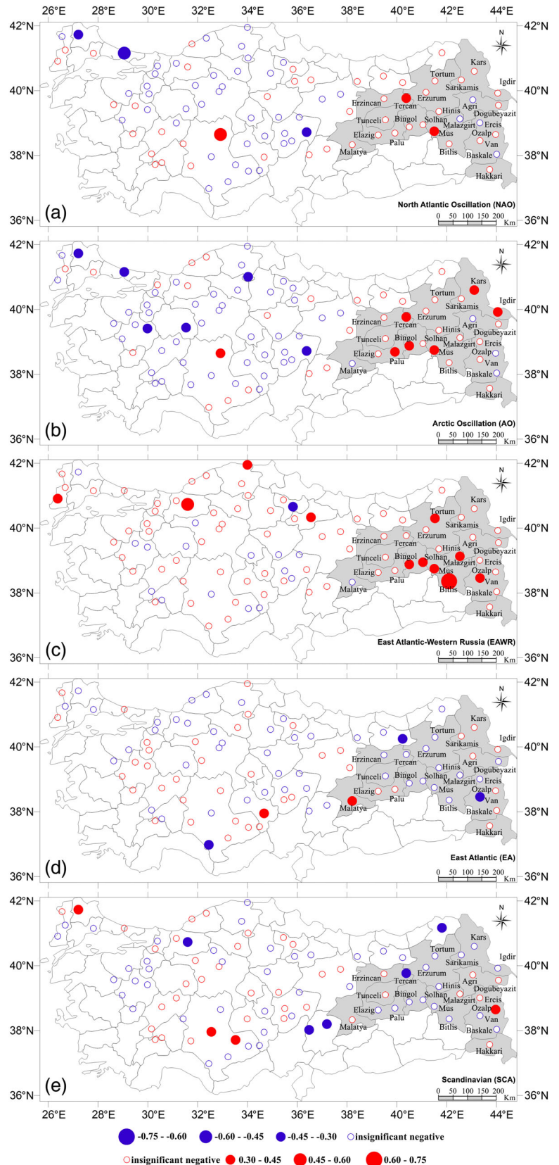
FIGURE 6 Correlation coefficients between extended winter (December to March) mean snow cover depth (SCD) and (a) North Atlantic Oscillation (NAO), (b) Arctic Oscillation (AO), (c) east Atlantic/western Russia (EA/WR), (d) east Atlantic (EA) and (e) Scandinavian (SCA) indices. The grey shaded area indicates the EAR with its station names
