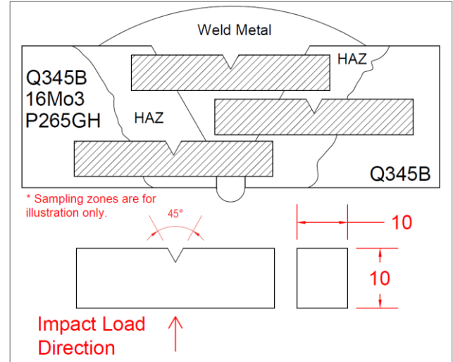
Figure 4. Impact tests for specimen types and test notch point (mm).
