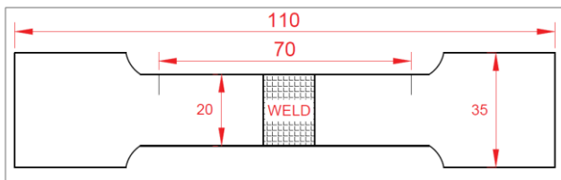
Figure 2. Tensile test specimen (mm) [35].
