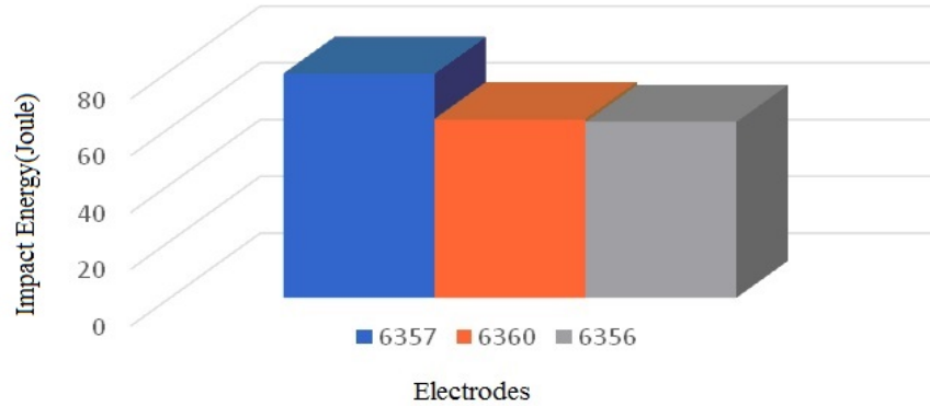
Figure 4. The impact energy of the welded samples with GeKa Tempo B 65 electrode.
