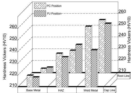
Figure 11. Hardness test results
