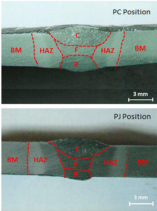
Figure 12. Macrostructure images
