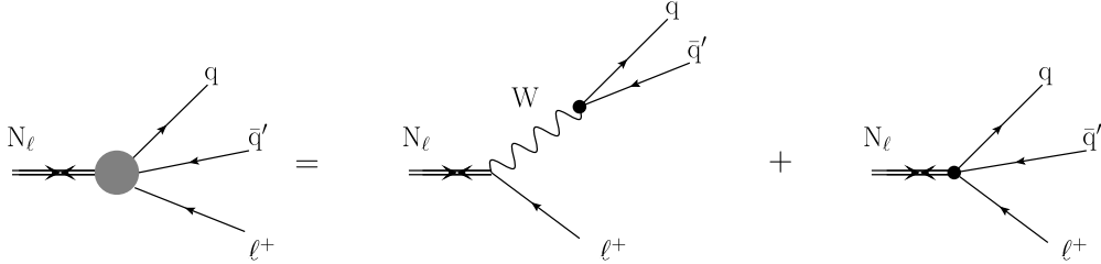
Fig. 2. Feynman diagrams for the decay of a heavy composite Majorana neutrino to \ell^+ q \bar{q}' .
