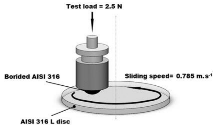
Figure 8. Schematic figure of pin-on disk friction test device
