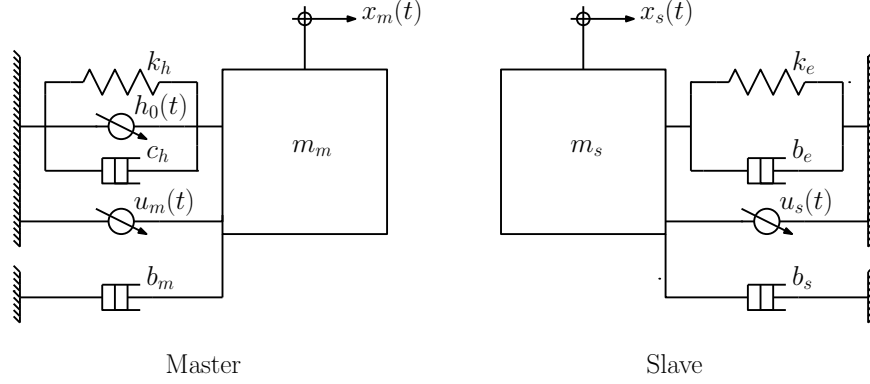
Figure 1: Bilateral teleoperation system
